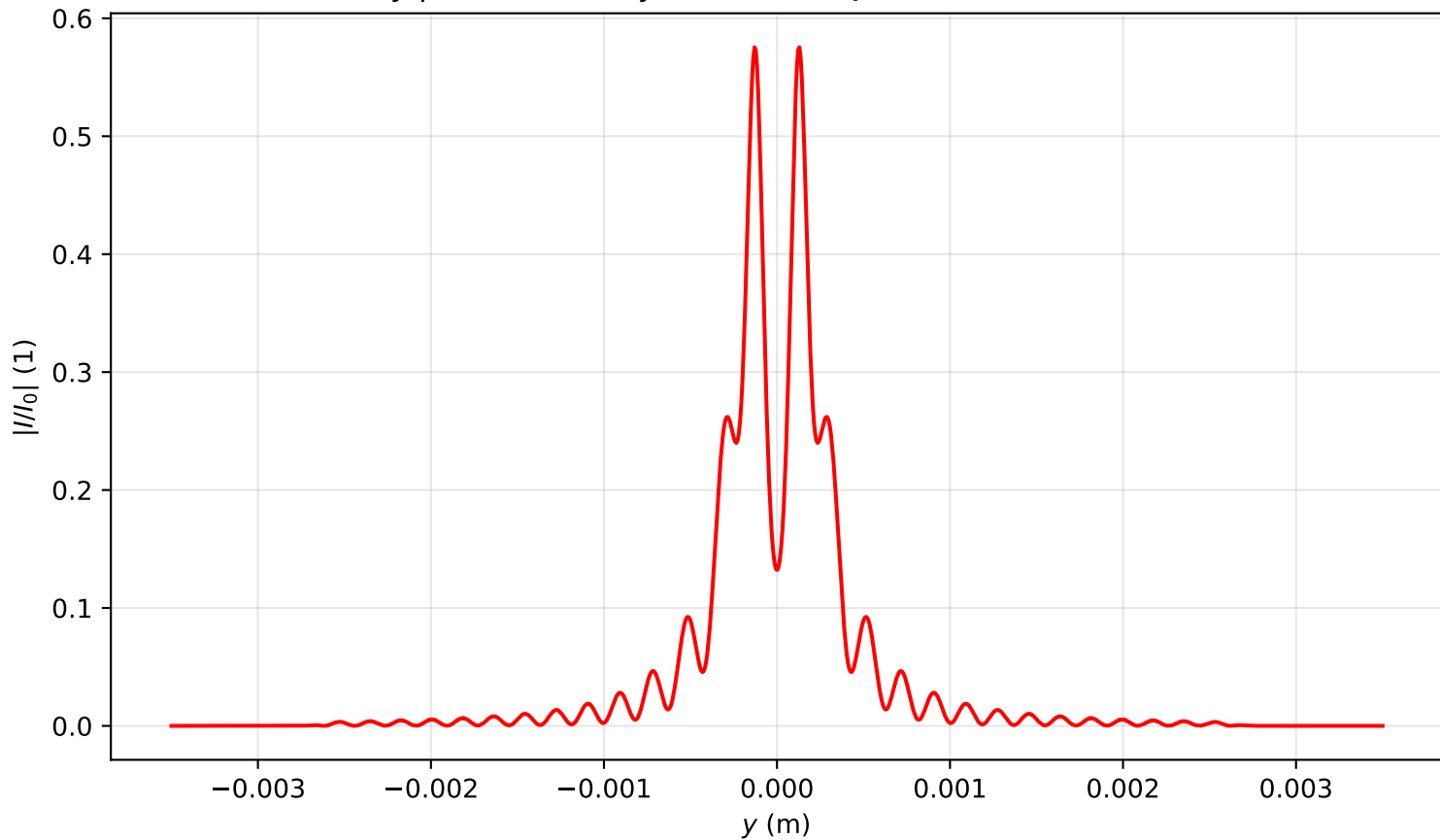
Intensity profile I(x=0, y, z=0.159)/I_0 , \text{Pin}=6.0\text{Pcr} , artificial time
